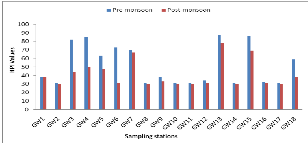
Figure 2: HPI values at various sampling points in pre and post monsoon season.
